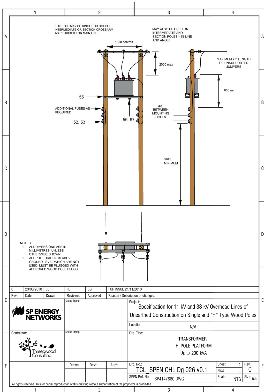
22.26 Figure 26 General Arrangement Transformer “H” Pole Platform up to 200kVA (Drawing No. SP4147880)
